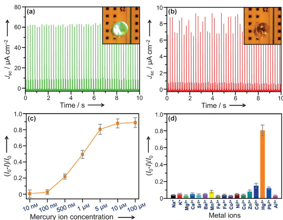
Figure 4. a,b) Rectified J_{\text{sc}} of the as-developed TENG before (a) and after (b) the interaction with 5\text{ }\mu\text{M} \text{Hg}^{2+} ions. Insets: photograph of the indicated LED lamp before (a) and after (b) interaction with 5\text{ }\mu\text{M} \text{Hg}^{2+} ions, as an indication of detected concentration. c) Sensitivity and d) selectivity of the as-developed TENG for the detection of \text{Hg}^{2+} ions. The concentration of all metal ions tested in the selectivity experiment was 5\text{ }\mu\text{M} .
